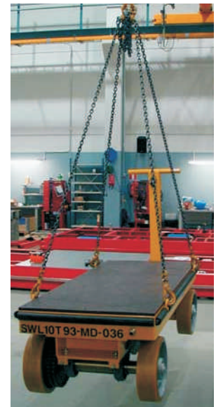
Lifting eye bolts allow the trolley to be lifted by crane.
